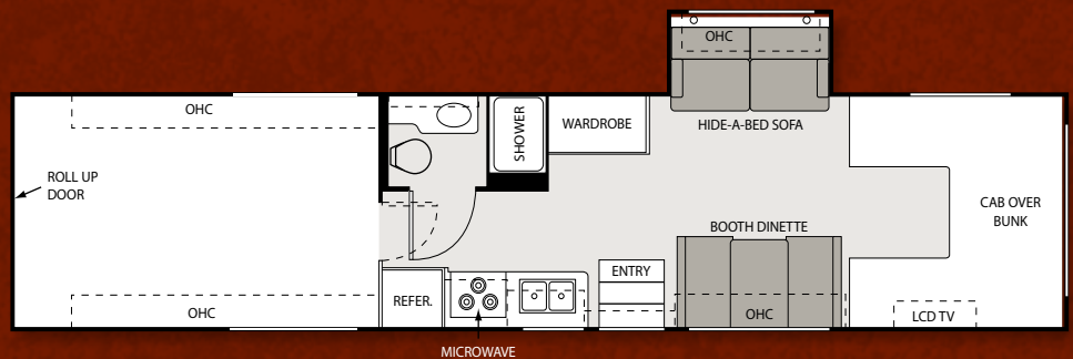
42C CARGO AREA: 96" x 163"
