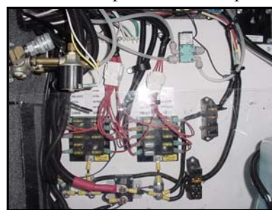
Figure 7-2. Fuse Panel
