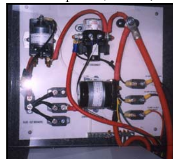
Figure 7-19. Circuit Breakers
