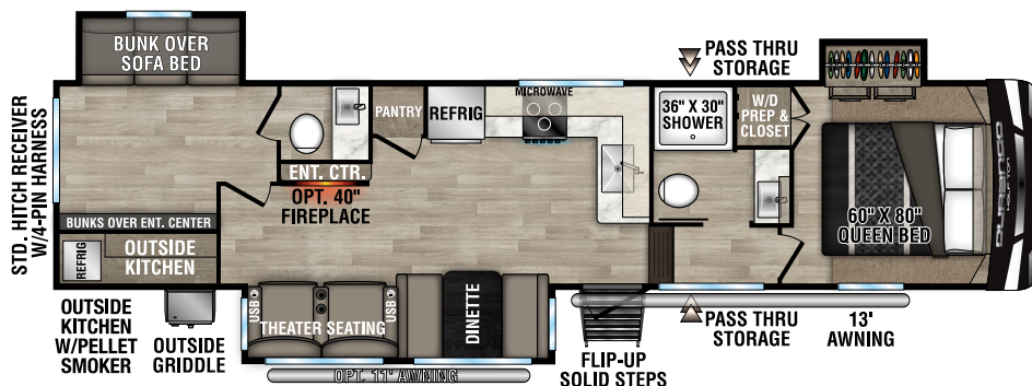
D291BHT UVW - 9,660 | Exterior Length - 37' 5" | Sleeps - 9
