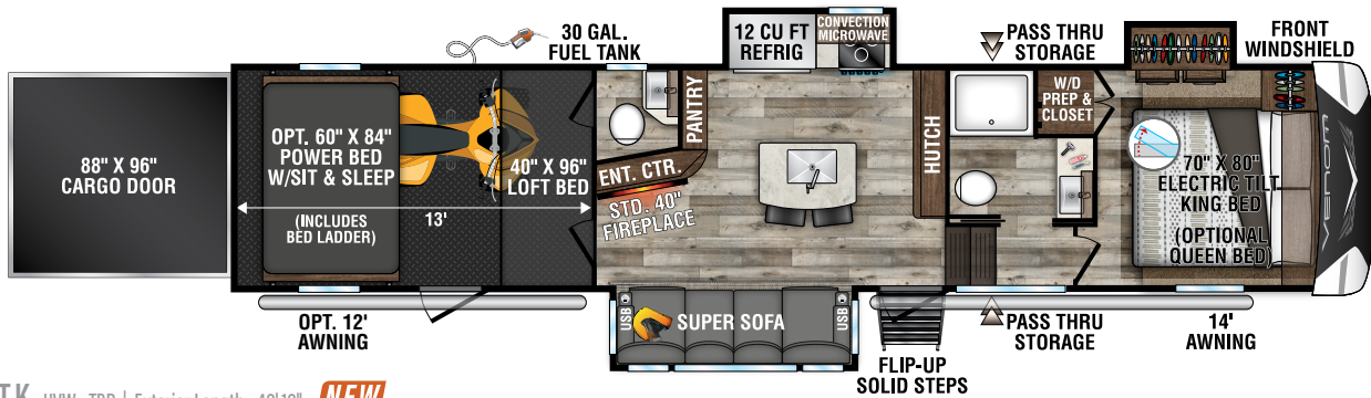
V3313TK UVW - TBD | Exterior Length - 40'10" NEW
