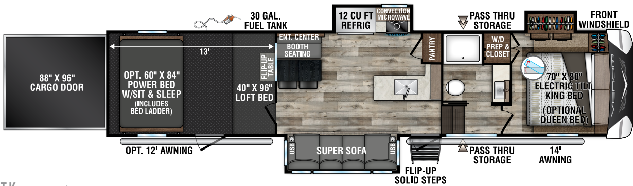
V3413TK UVW - 12,740 | Exterior Length - 40'11"
