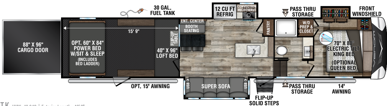
V3916TK UVW - 13,340 | Exterior Length - 43'8"
